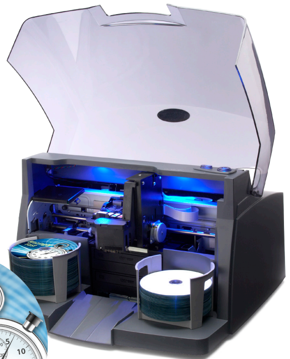
Bravo 4102 Disc Publisher
